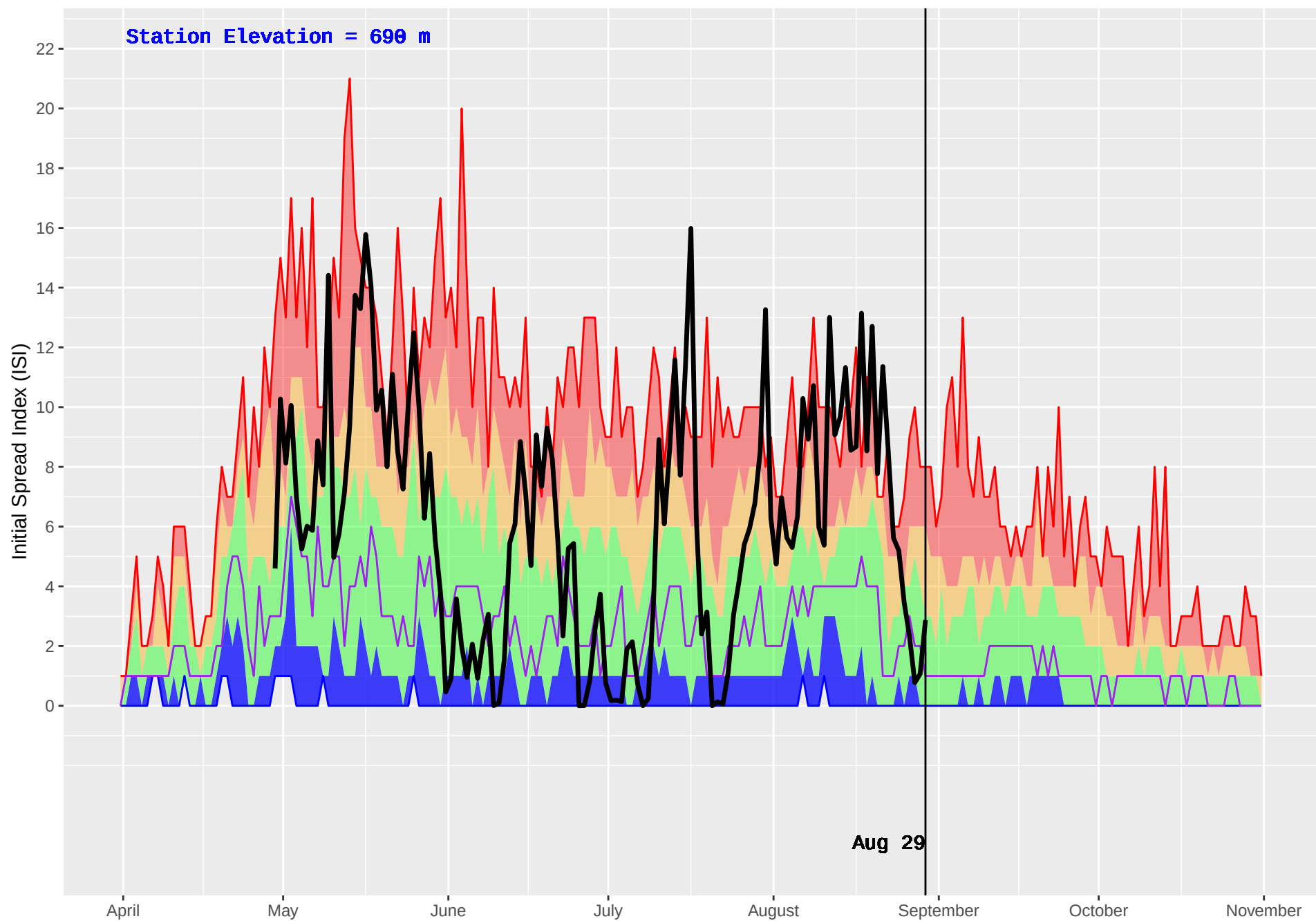
MACKENZIE FS (155) : Historical (1994–2016) and Current (2018) Daily Initial Spread Index (ISI)
