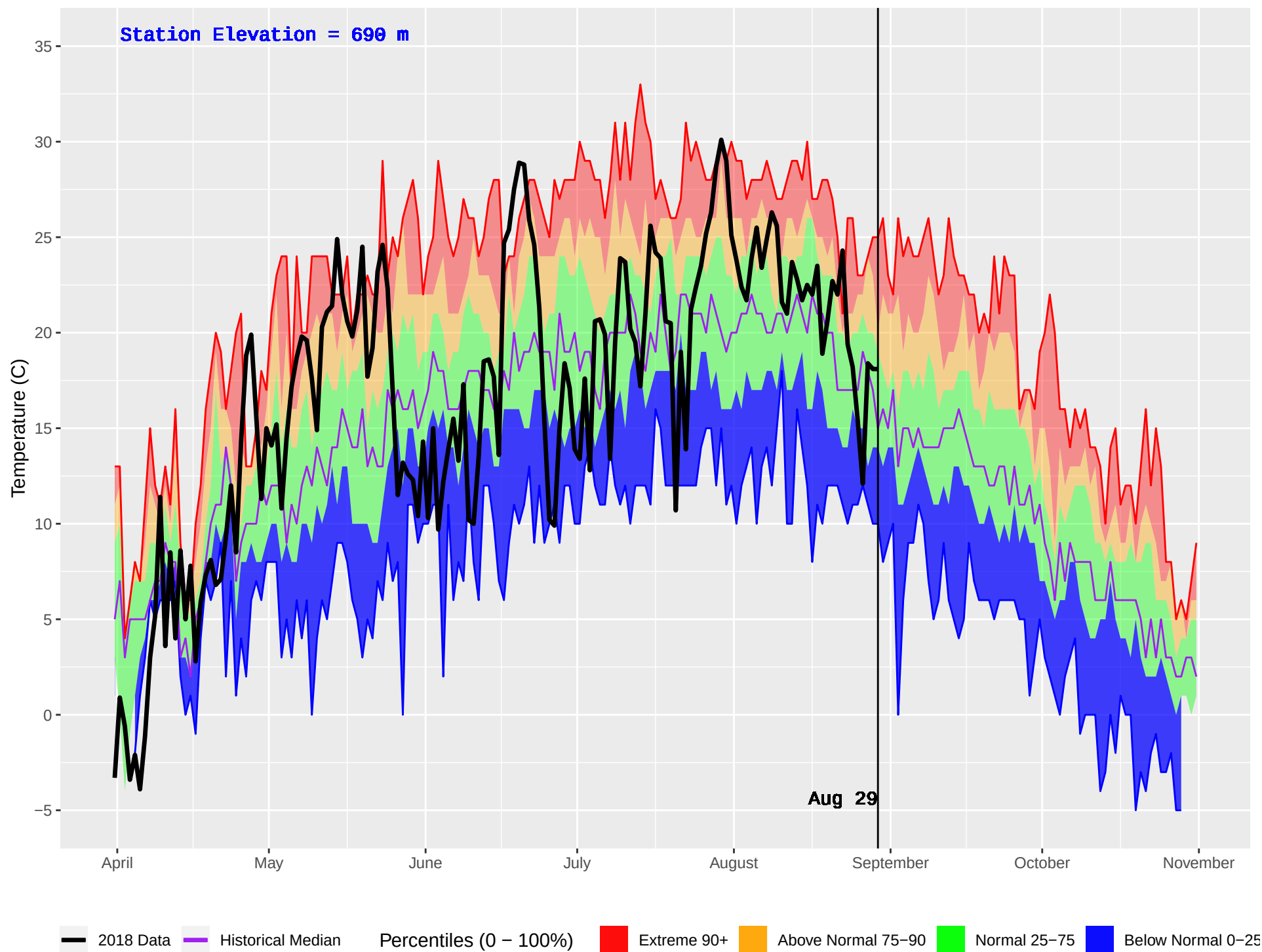
MACKENZIE FS (155) : Historical (1994–2016) and Current (2018) Daily Temperature
